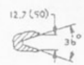
SECTION F-F DETAIL OF PULLEY GROOVES SCALE: 1=1
