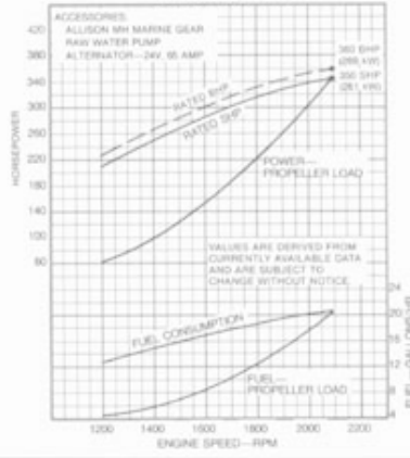
MODEL 8V-92 MARINE INTERMITTENT RATING 9280 INJECTORS*
