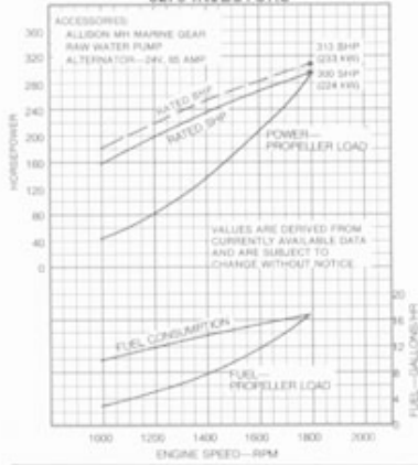
MODEL 8V-92 MARINE CONTINUOUS RATING 9275 INJECTORS*
