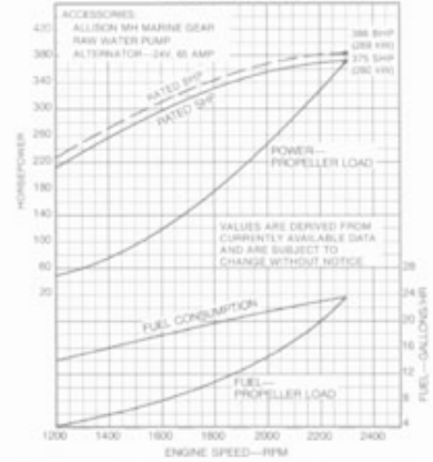
MODEL 8V-92 MARINE MAXIMUM RATING 9285 INJECTORS*
